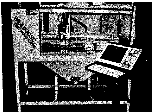
Servo Version with optional C- Axis 3-Axis CNC Wood Lathe
